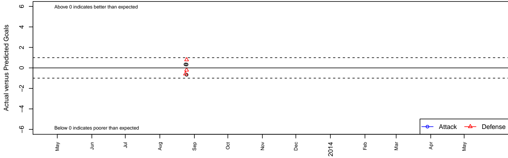
Scorpions G00 Dots are actual minus expected GF (blue circles) and GA (red triangles). Blue line is smoothed change in attack strength. Red is smoothed change in defense strength.
